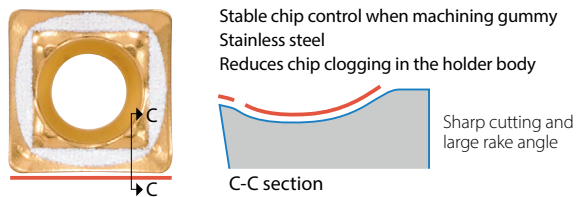
For stainless steel machining: SM chipbreaker
