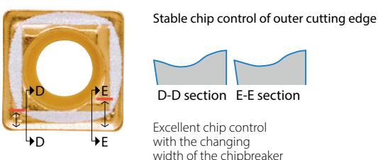
For machining soft steel and SS material: XM chipbreaker
