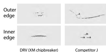
Chip control comparison (In-house evaluation)
