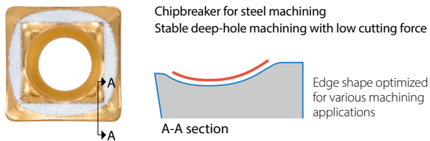
General purpose: GM chipbreaker
